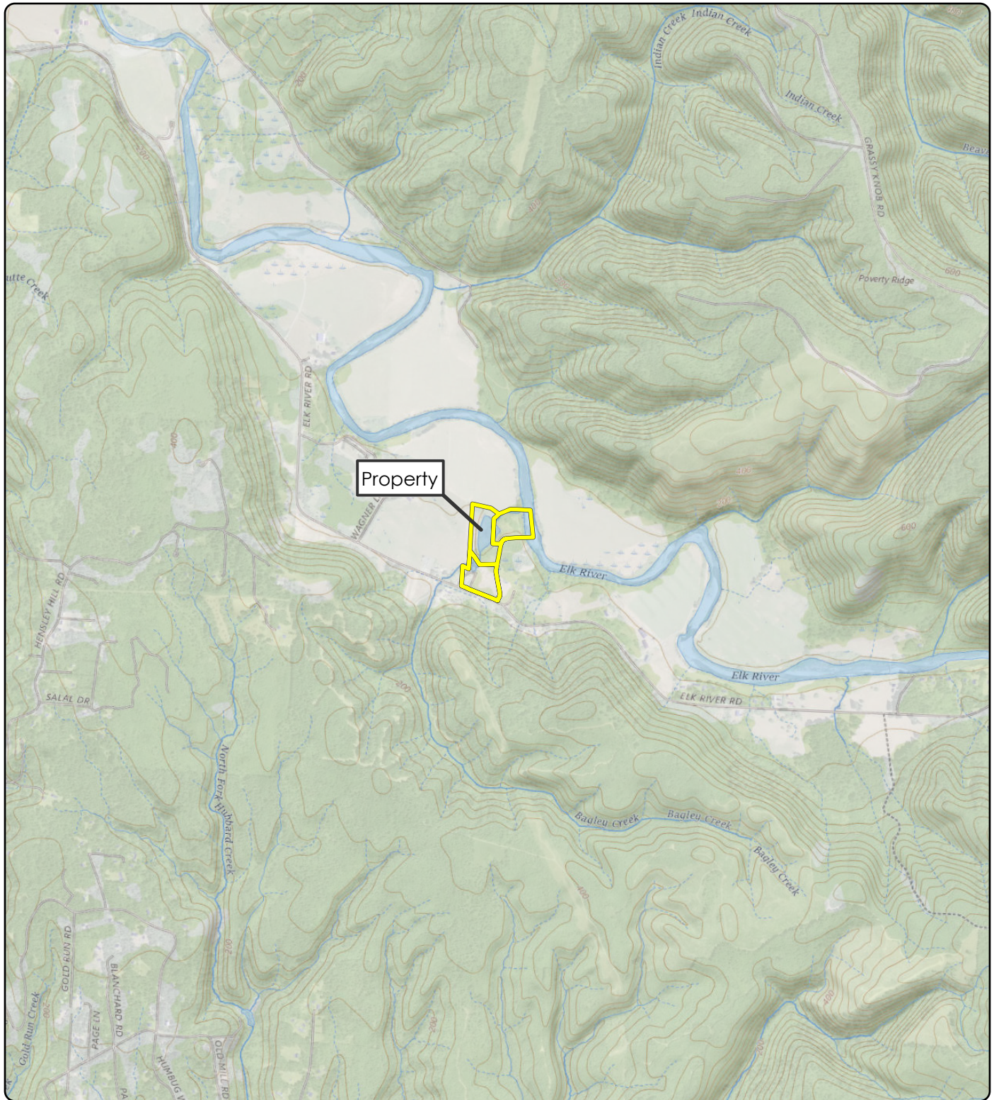
Figure 2-1 Vicinity Map
